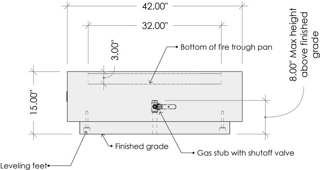
FRONT VIEW
