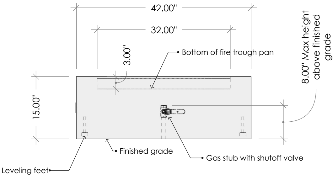
FRONT VIEW
