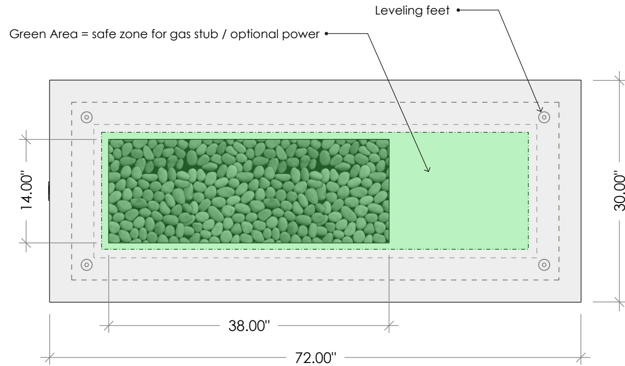
TOP VIEW
